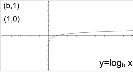
Log
