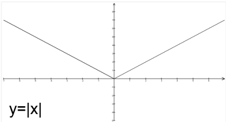
Absolute Value
