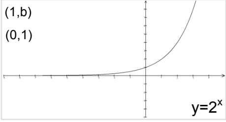
Exponential
